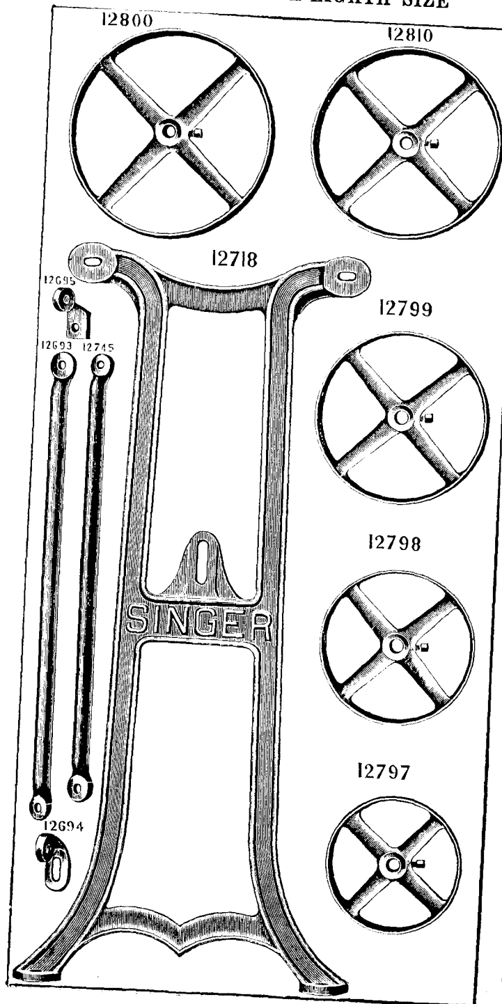
PLATE 1078-ONE-EIGHTH SIZE
