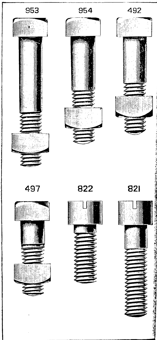
PLATE 1060--FULL SIZE
